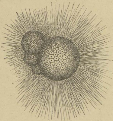
FIG. 6.—Foraminifer, Globigerina bulloides , magnified seventy diameters. This form is found floating in tropical and temperate seas.
