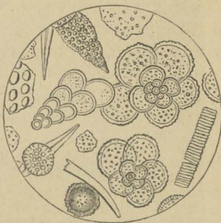
FIG. 8.—Organisms in Atlantic Ooze (highly magnified).
