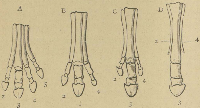
FIG. 21.—Feet of Ancestors of the Horse ( Equidæ ).
