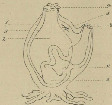
FIG. 55. — Diagram of Structure of Sea-squirt.
