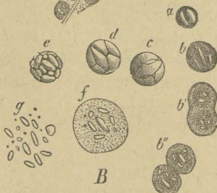
FIG 63.—Chlorophyll Granules in Leaf-cells (magnified 550 diameters).
