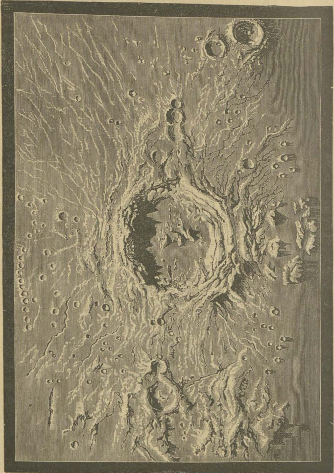
FIG. 2.—Lunar Crater : Copernicus.
