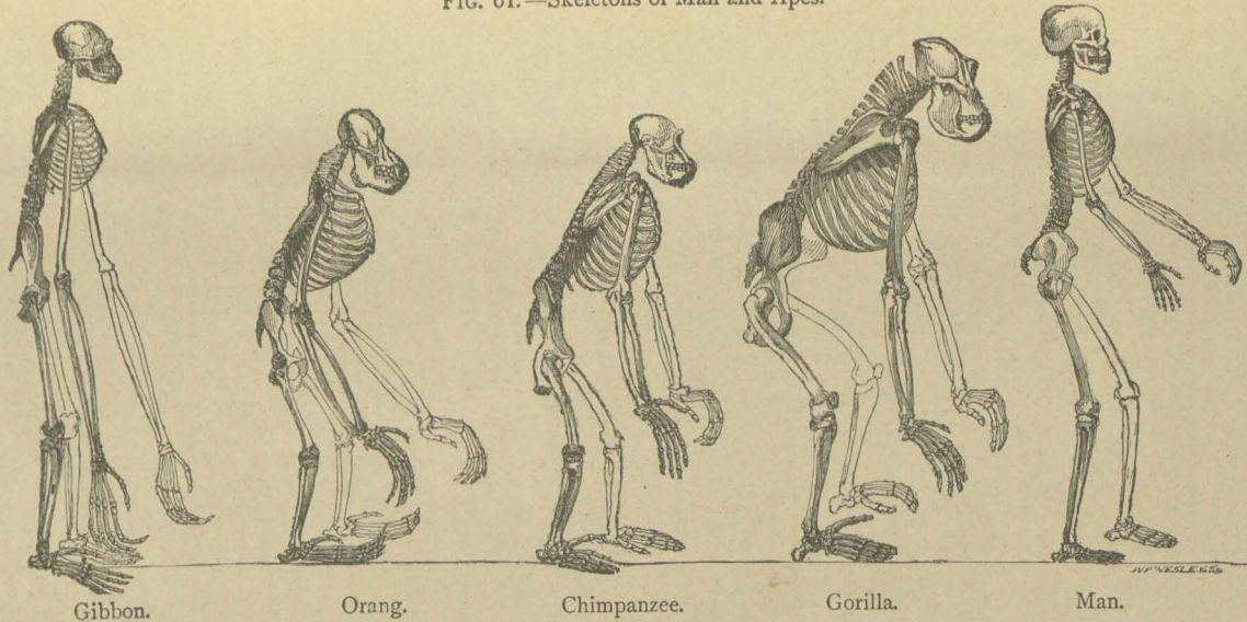
FIG. 61.—Skeletons of Man and Apes.
