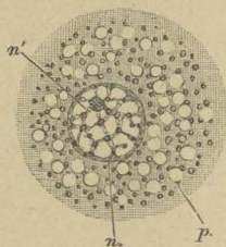
FIG. 27.—Diagram of a Cell.
