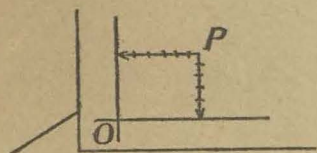
Fig. 5.—To locate P on a plane we measure from P to each of two axes at right angles, thus obtaining two numbers.
